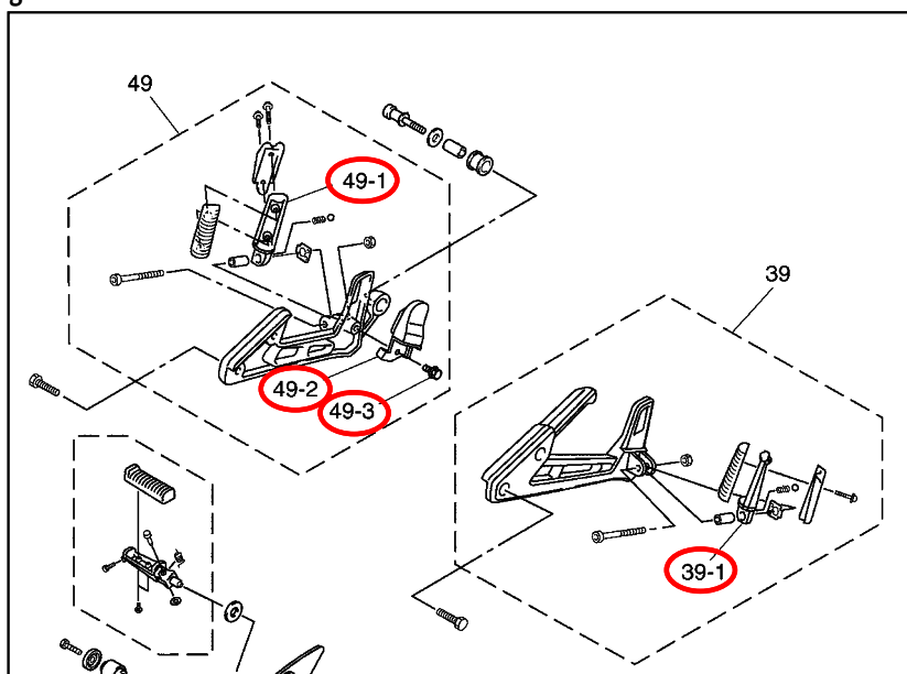
Fig.35 STAND. FOOTREST
