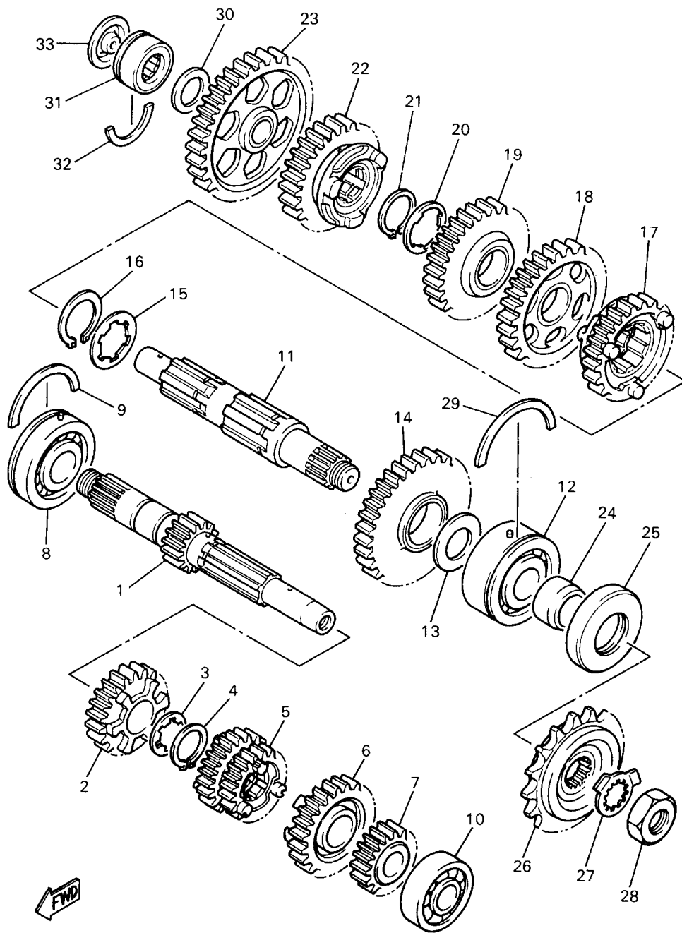
FIG. 17 TRANSMISION
